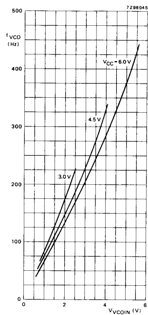
Fig. 17 Graphs showing VCO frequency ( f_{VCO} ) as a function of the VCO input voltage ( V_{COIN} ).
